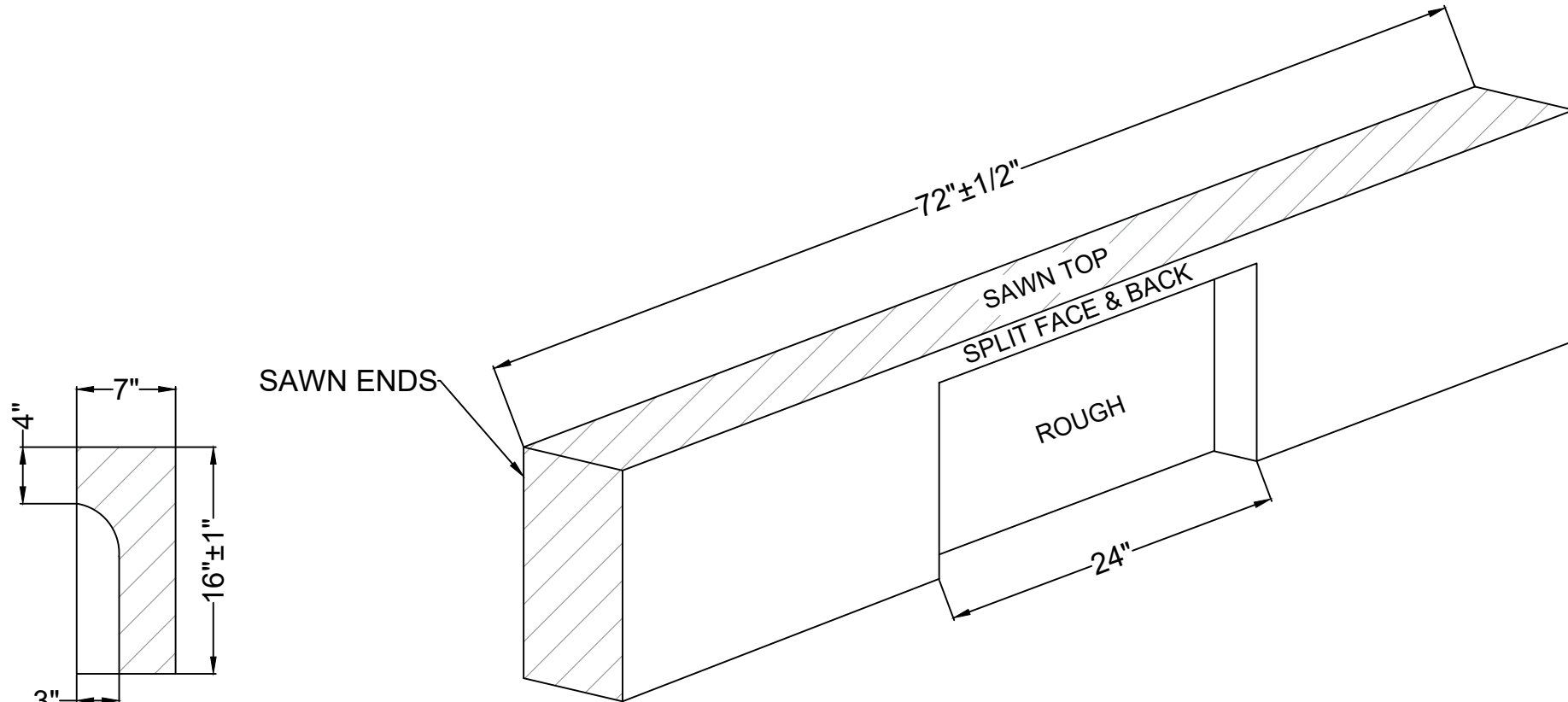
SECTION VIEW
