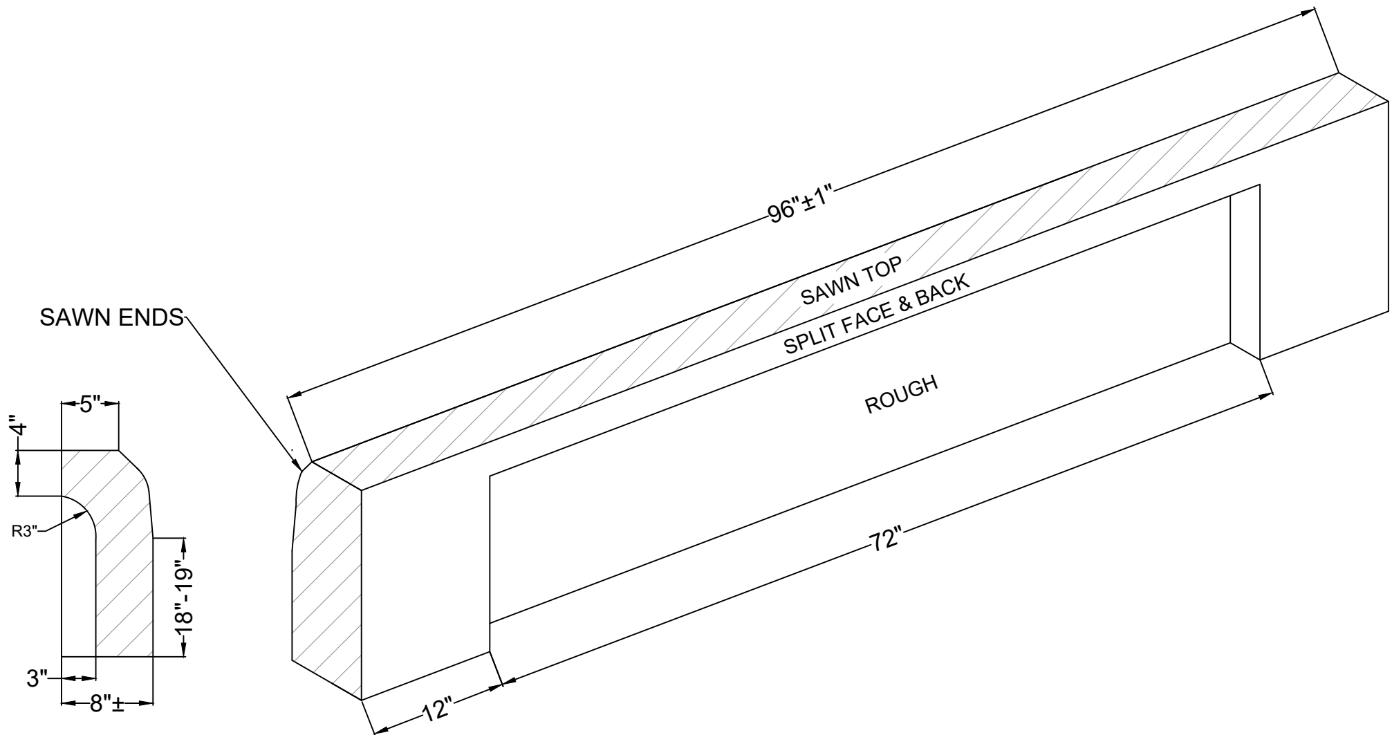
SECTION VIEW
